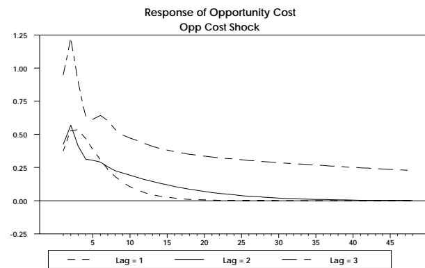
Figure 3 Impulse Response Functions
